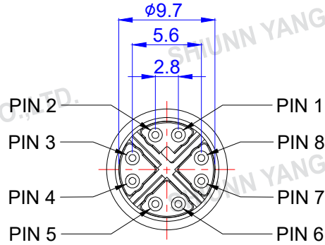
A : M12 X-CODE 8PIN MALE
