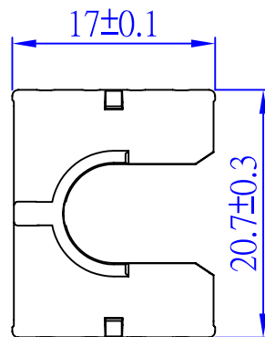
wire cover
